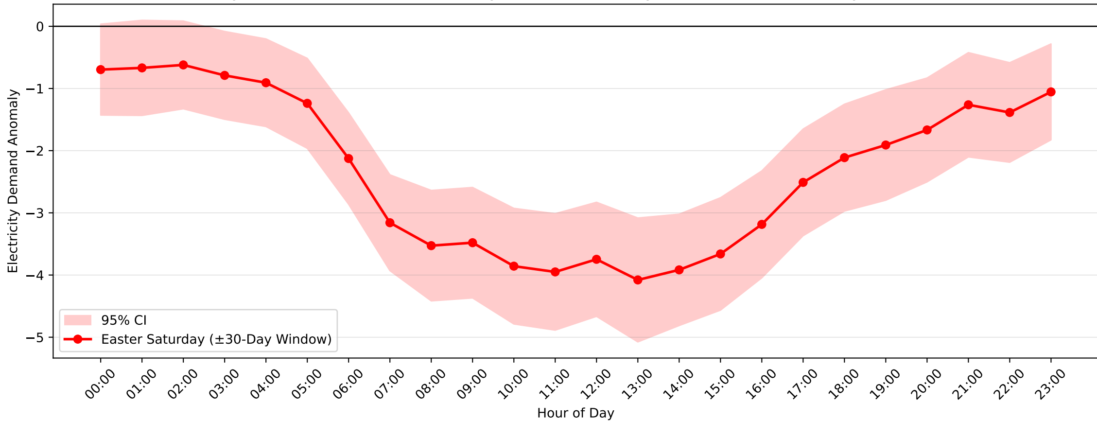
Mayfield West Demand Anomaly: Easter Saturday (2004-2017, \pm 30 -Day Window)
